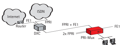
TYPICAL APPLICATION: DELIVERING COMBINED ISDN, FE1 AND IP SERVICES
