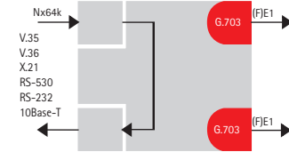
FIGURE3: NX64K INTERFACE CONVERTER
